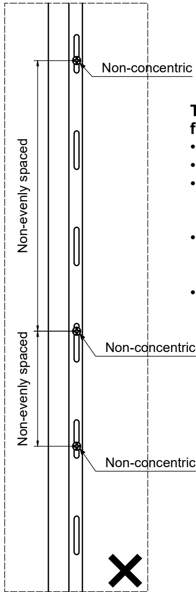
Incorrect screwing
