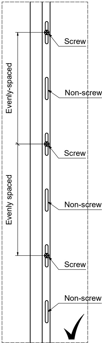
Correct screwing
