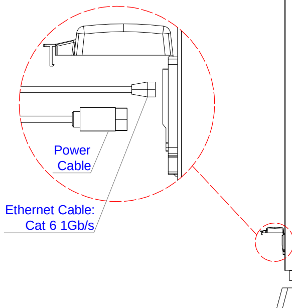
Pod Power Input
